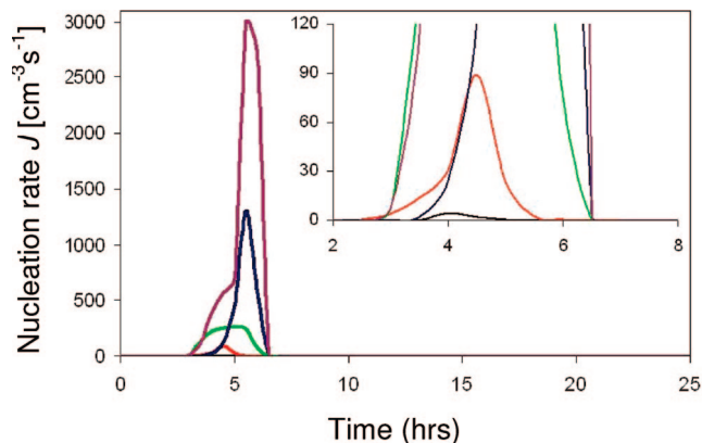
Figure 4. Deduced nucleation rate J of lysozyme in the presence of 0.5 M NaCl and 0.05 M NaAc at pH 4.5, as a function of time. The inset is a close-up of the main graph. The different curves describe J for different quench profiles (online in color).
