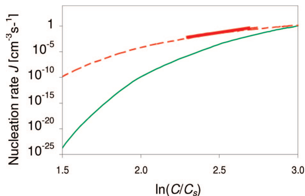
Figure 6. Crystal nucleation rate J as a function of supersaturation. Solid (thin) green curve: nucleation rates calculated using our fitting parameters A = 6.2 \times 10^5 \text{ mg}^{-1} \text{ s}^{-1} and B = 160 (extracted from a crystallization experiment with initially 3.5% NaCl), for protein solubility C_s = 5 \text{ mg/mL} and a range of protein concentrations (20 mg/mL to 100 mg/mL). Dashed red curve: nucleation rates calculated using the fitting constants of Galkin and Vekilov ( A = 18 \text{ mg}^{-1} \text{ s}^{-1} and B = 65 , extracted from a crystallization experiment with 2.5% NaCl). Solid (thick) red curve: experimental data of Galkin and Vekilov at C_s = 5 (online in color).
